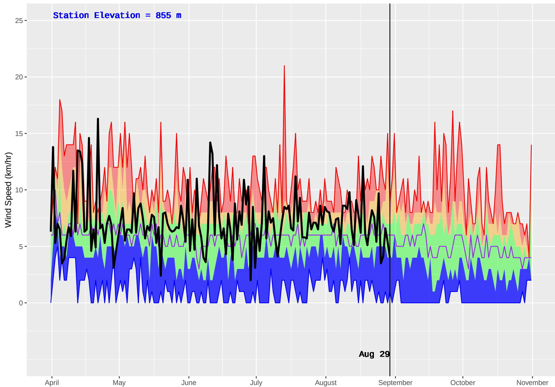
AUGUST LAKE (836) : Historical (2003–2016) and Current (2018) Daily Wind Speed
